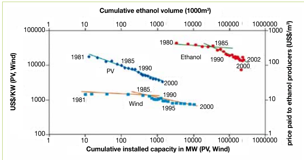
Figure 16: Technology Learning Curves
