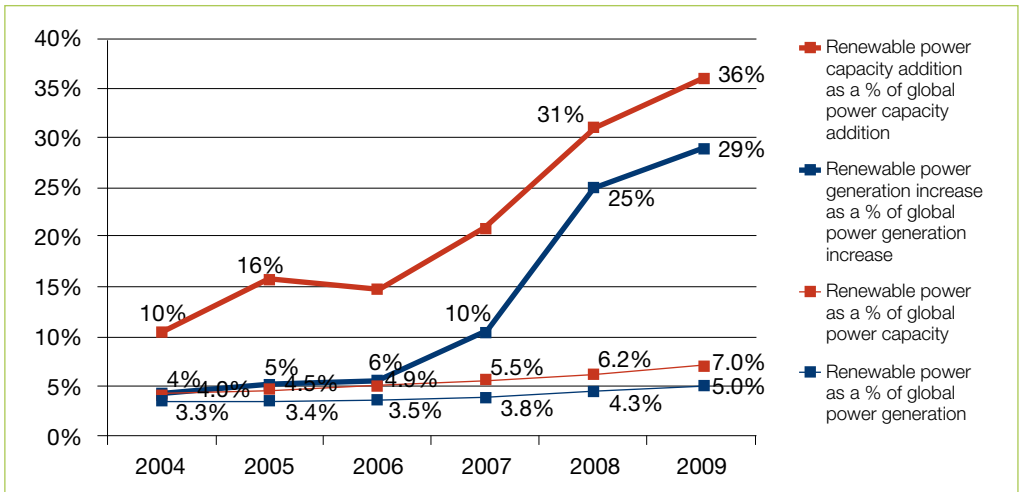
Figure 3: Global Growth of Renewable Energy in the Power Sector (excluding Large Hydro)
