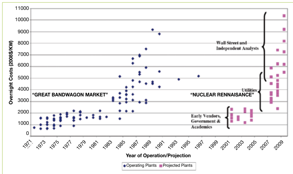
Figure 14: Investment Cost Evolution (“Learning Curve”) of US Nuclear Power Plants
