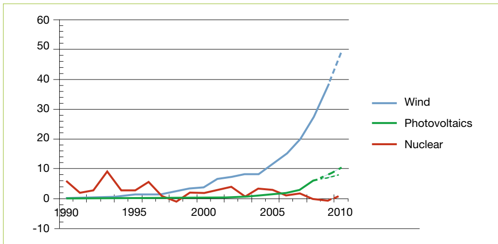
Figure 10: Net Additions to Global Electricity Grid from New Renewables and Nuclear 1990-2010 (in GW)
