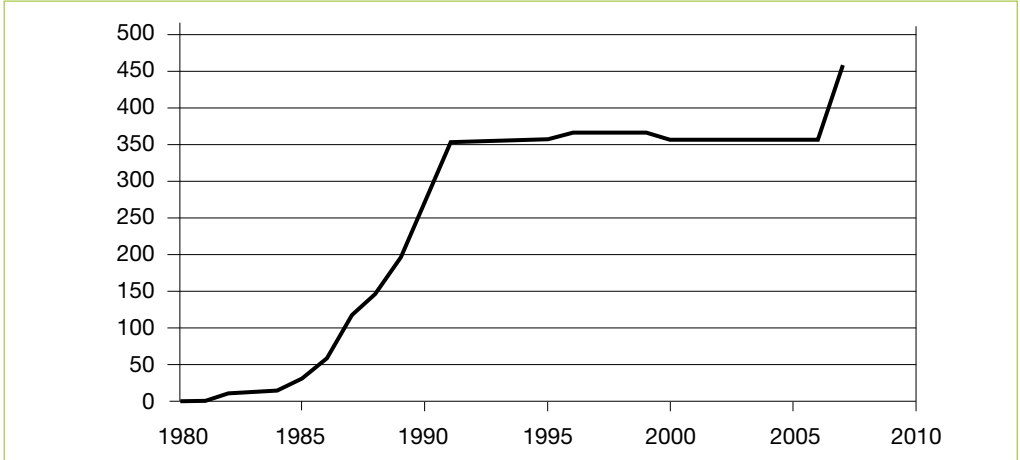
Figure 7: World Installed Concentrating Solar Thermal Power Capacity 1980-2007 (MW)
